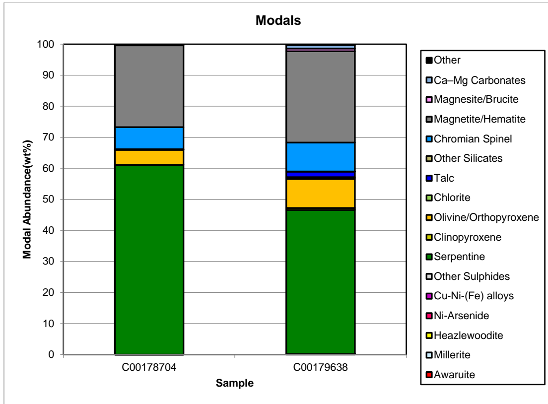
Figure 13-2: Modal Abundance of Minerals from QEMSCAN
