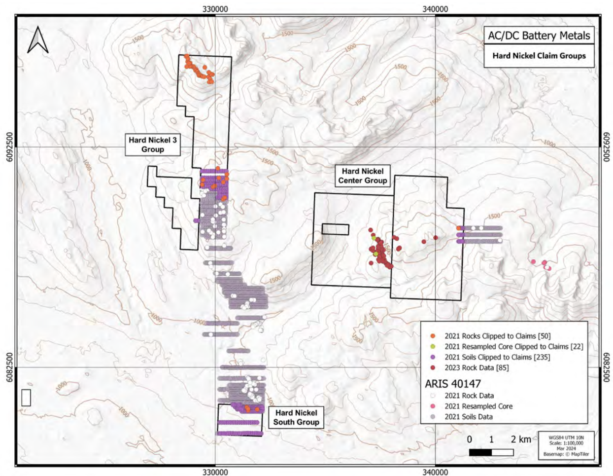
Figure 6-1: 2021 Samples Relative to Current Claims
