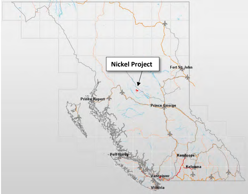
Figure 4-1: Location Map (BC view, 1:12,500,000 scale)
