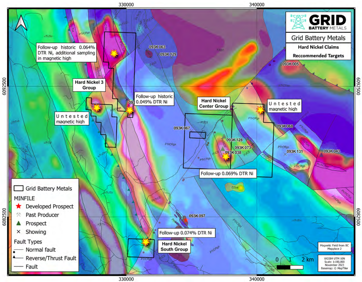
Figure 26-1: Nickel Project Exploration Targets
