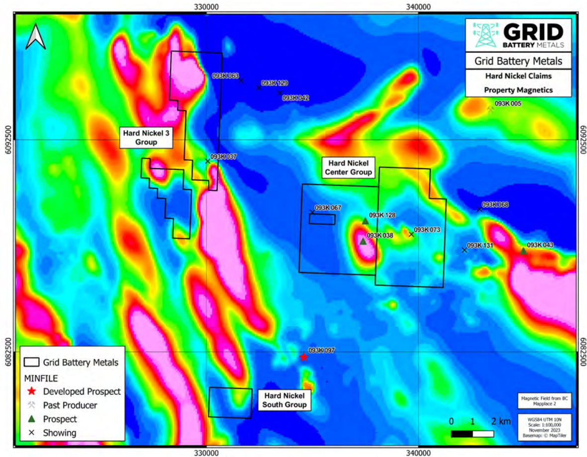
Figure 9-1: Regional Magnetics map for Nickel Project.
