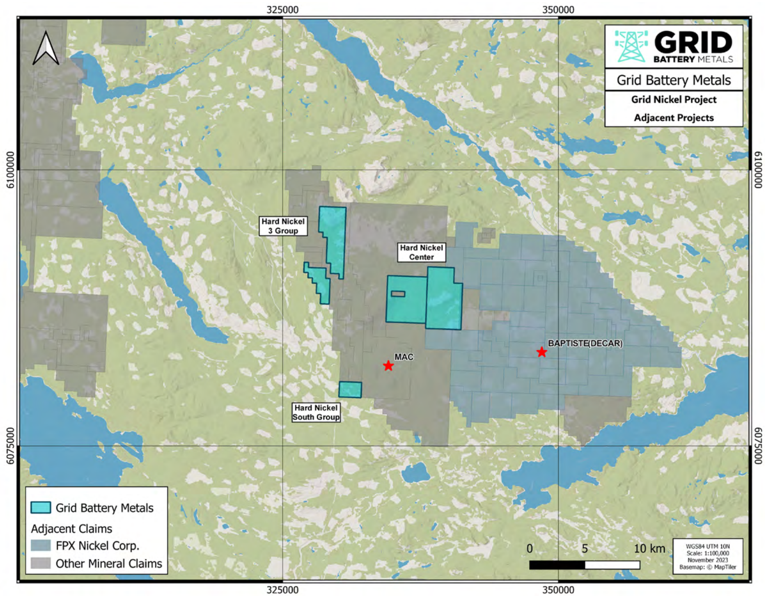
Figure 23-1: Decar Project in relation to Nickel Project claims
