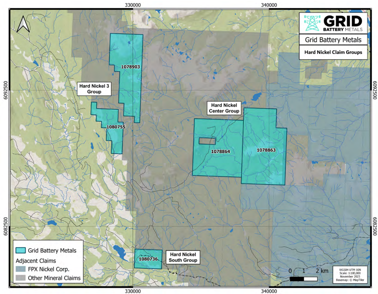
Figure 4-2: Nickel Property Claims Map (Central BC)
